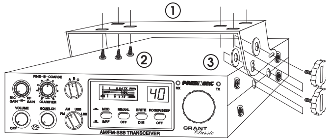
MOUNTING DIAGRAM
