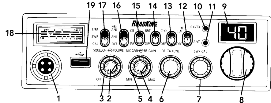
FRONT VIEW - RK5640 BACKLIGHTED PANEL
