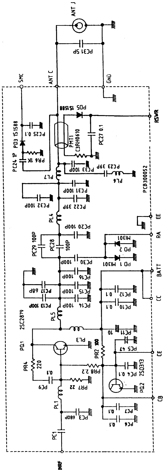
SUPERSTAR70000X POWER UNIT CIRCUIT
